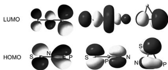
Figure 4. Molecular orbital plots (isovalue = 0.04) of the HOMO and LUMO for SNP, SPN, and cyc-PSN at the CCSD(T)/cc-pVTZ level of theory.
